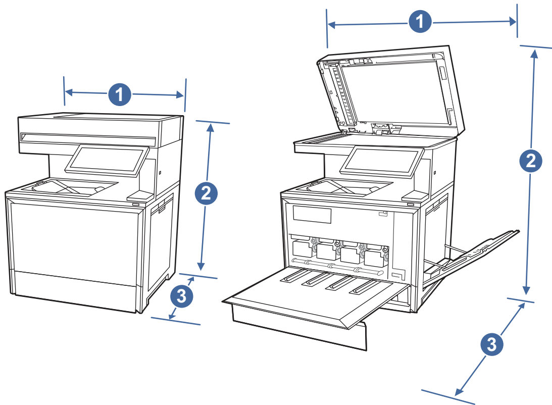
Figure 1-9 Printer dimensions (dn model)
