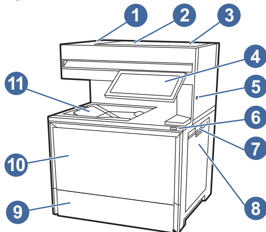
Figure 1-6 Printer front view
