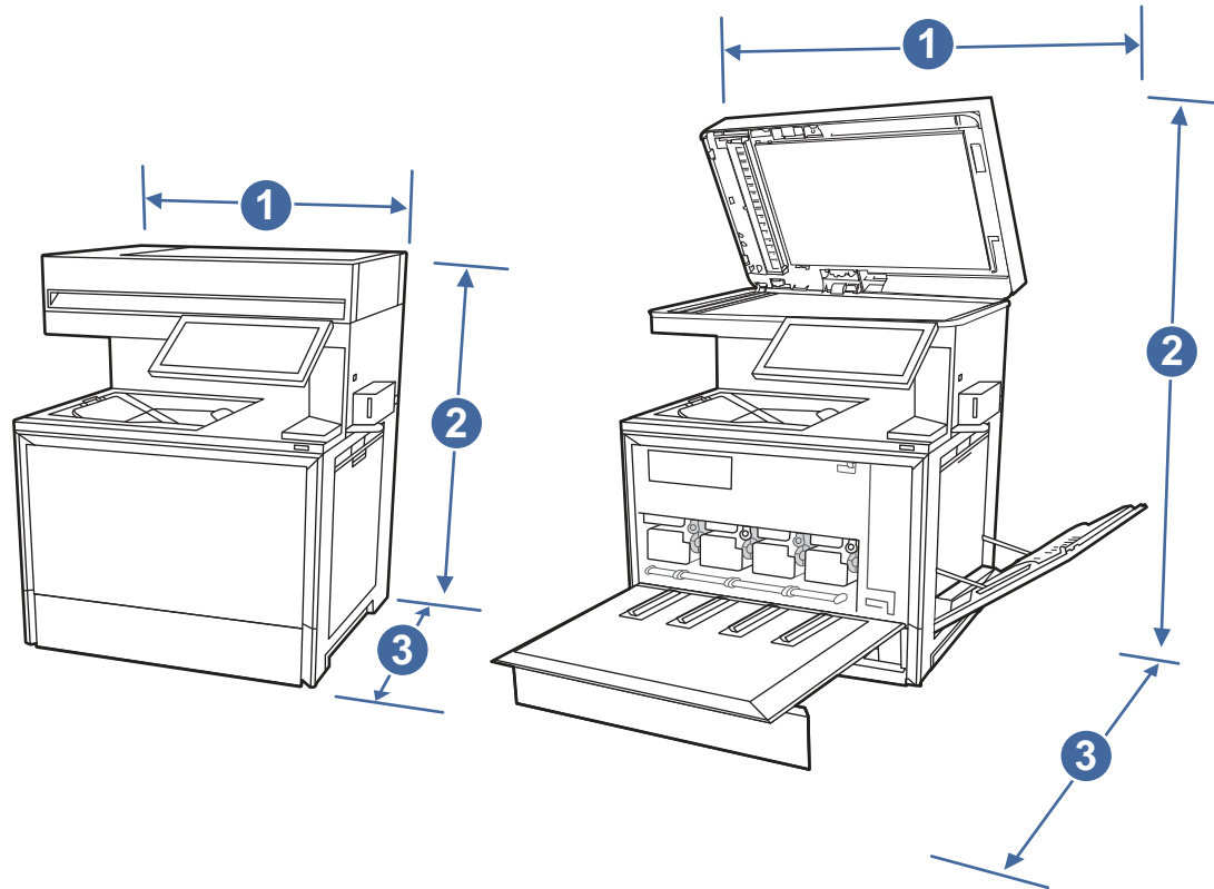
Figure 1-10 Printer dimensions (f and zf models)
