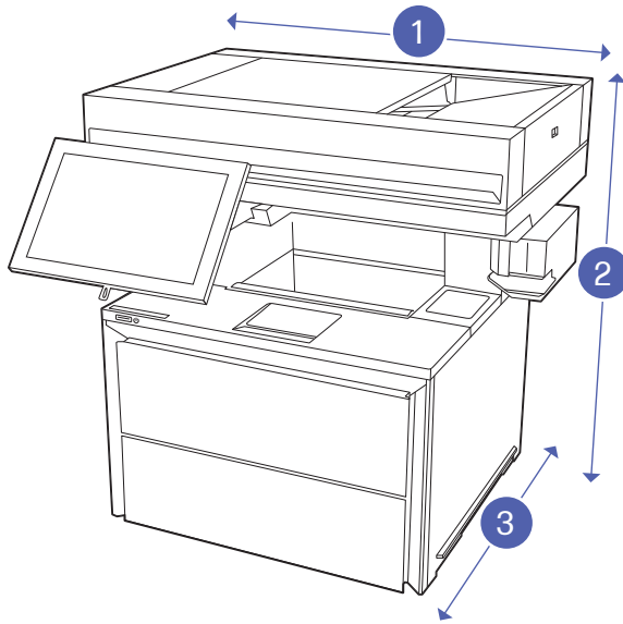
Figure 1-14 Dimensions for the printer opened
