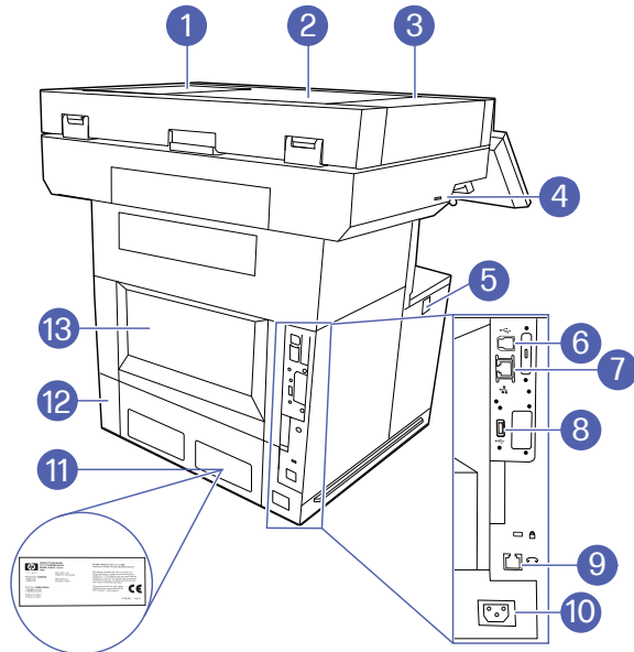
Figure 1-8 Printer rear view - X53052, X53052dn, X53052z
